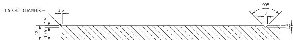
TYPICAL CHAMFER AND V-GROOVE DETAILS | SCALE 1:1
